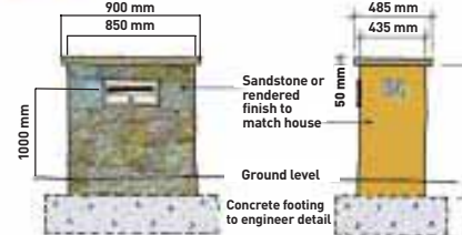
Driveway elevation
